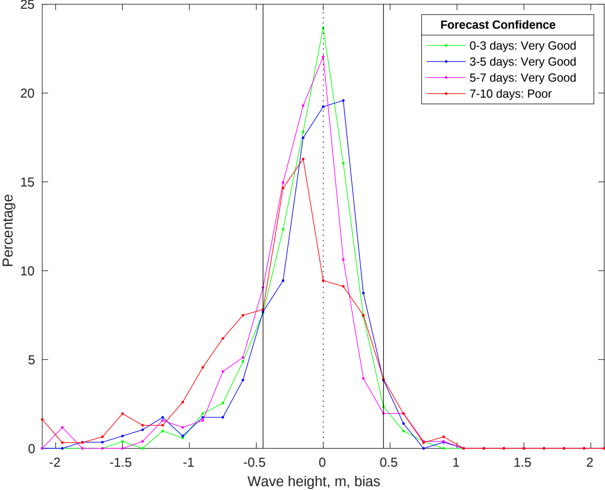
NDBC 51000 vs CMEMS Waves Bias Histogram: 24-Jan-2026
