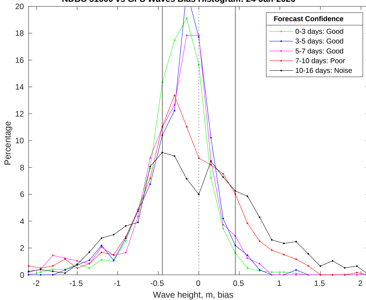
NDBC 51000 vs GFS Waves Bias Histogram: 24-Jan-2026
