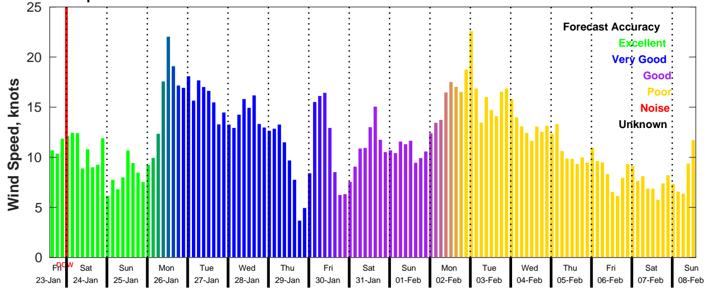
GFS Wind Speed Forecast for NDBC 51000 from 23-Jan-2026 14:00:00 to 08-Feb-2026 14:00:00
