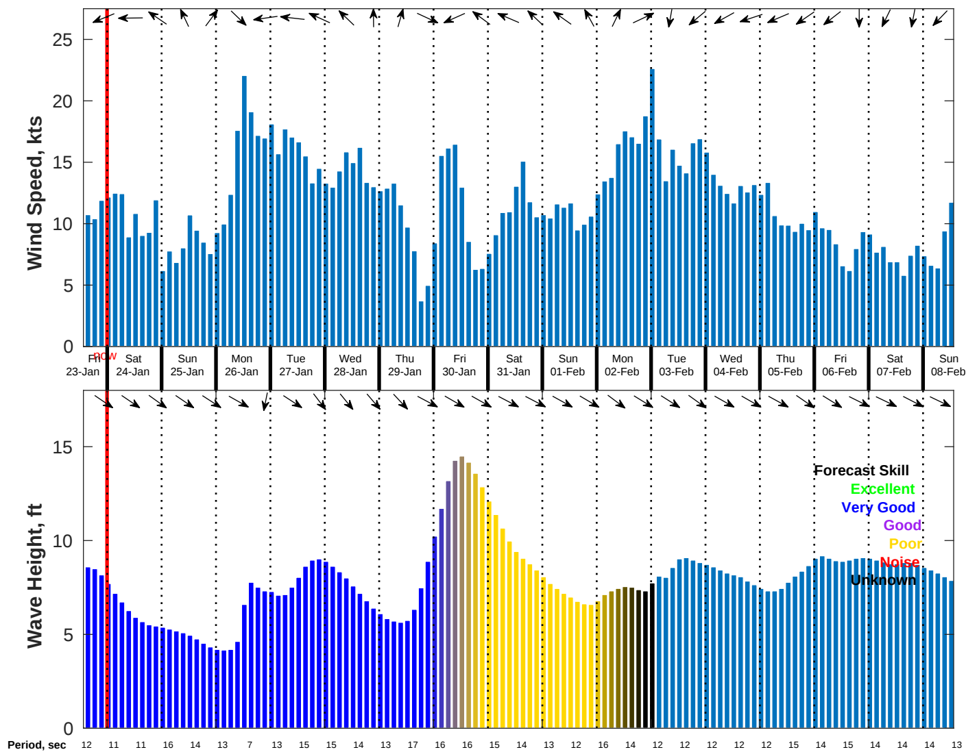
Wind & Wave Forecast for NDBC 51000 from 23-Jan-2026 14:00:00 to 08-Feb-2026 14:00:00
