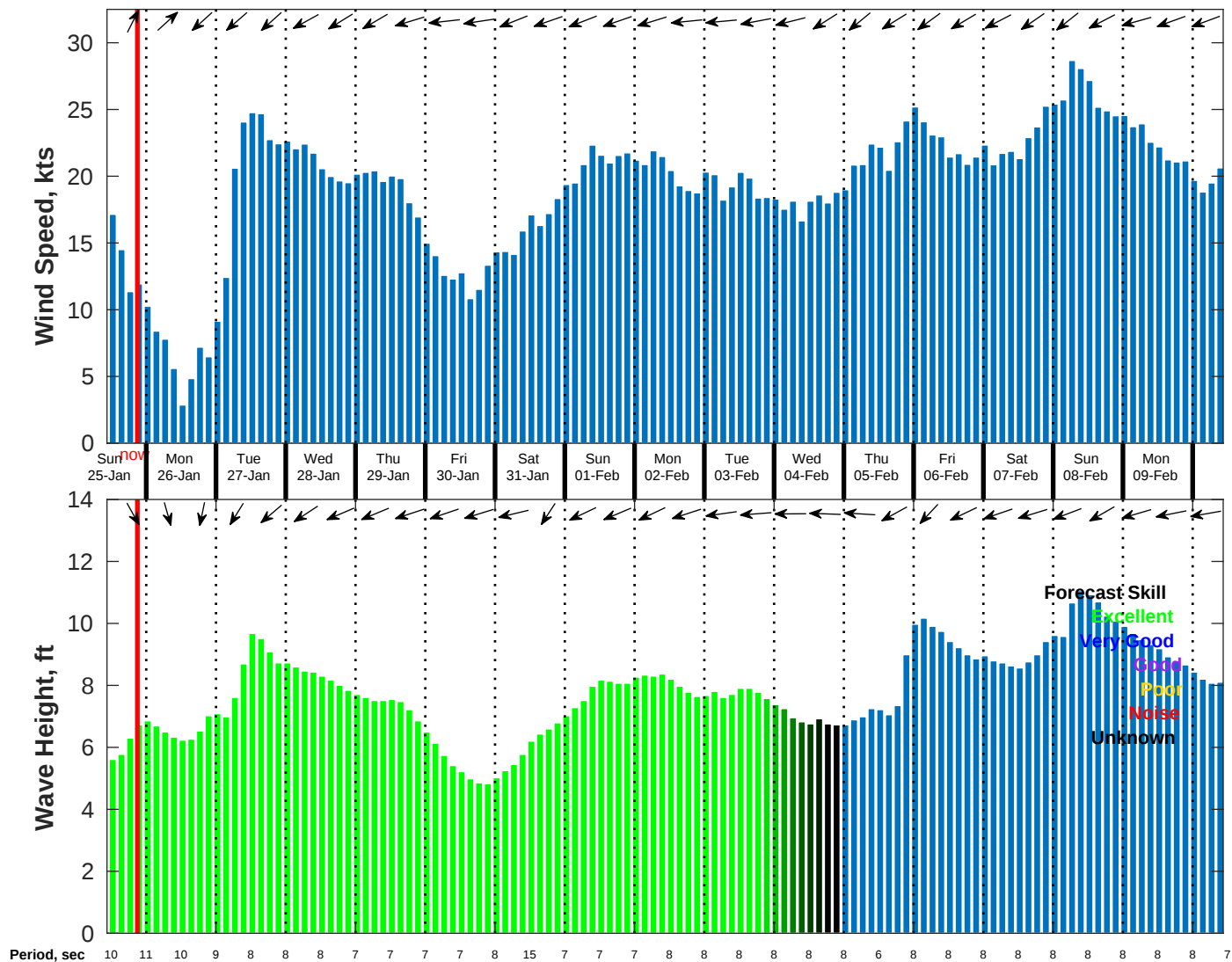
Wind & Wave Forecast for NDBC 52211 from 24-Jan-2026 11:00:00 to 09-Feb-2026 11:00:00
