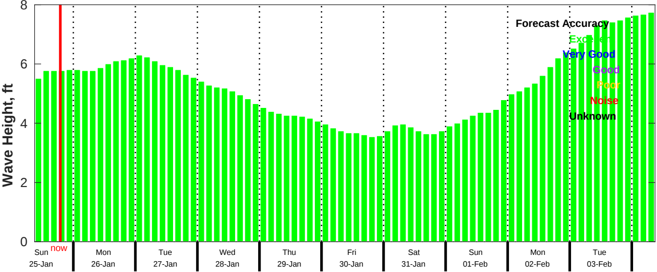
CMEMS Wave Forecast for NDBC 52212 from 24-Jan-2026 09:00:00 to 03-Feb-2026 09:00:00
