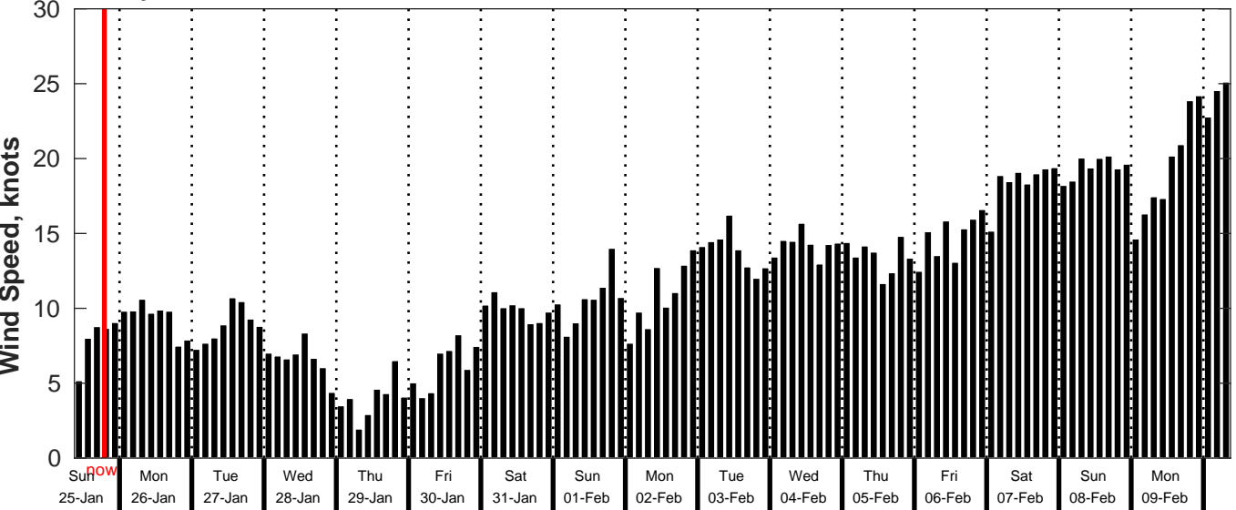
GFS Wind Speed Forecast for NDBC 52212 from 24-Jan-2026 09:00:00 to 09-Feb-2026 09:00:00
