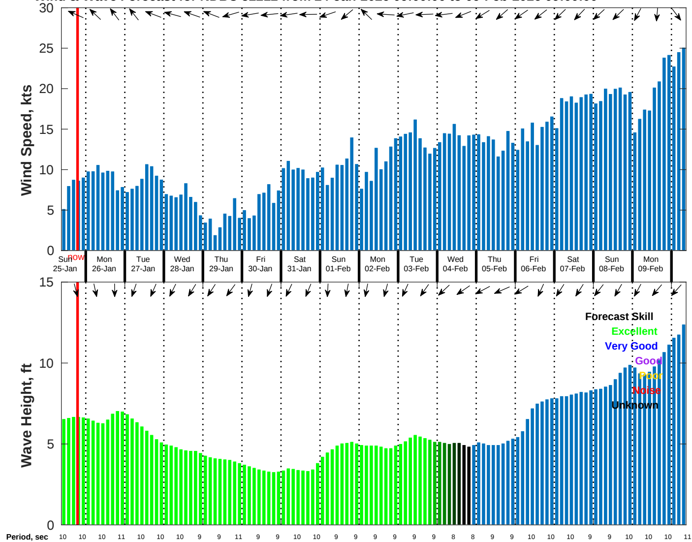
Wind & Wave Forecast for NDBC 52212 from 24-Jan-2026 09:00:00 to 09-Feb-2026 09:00:00
