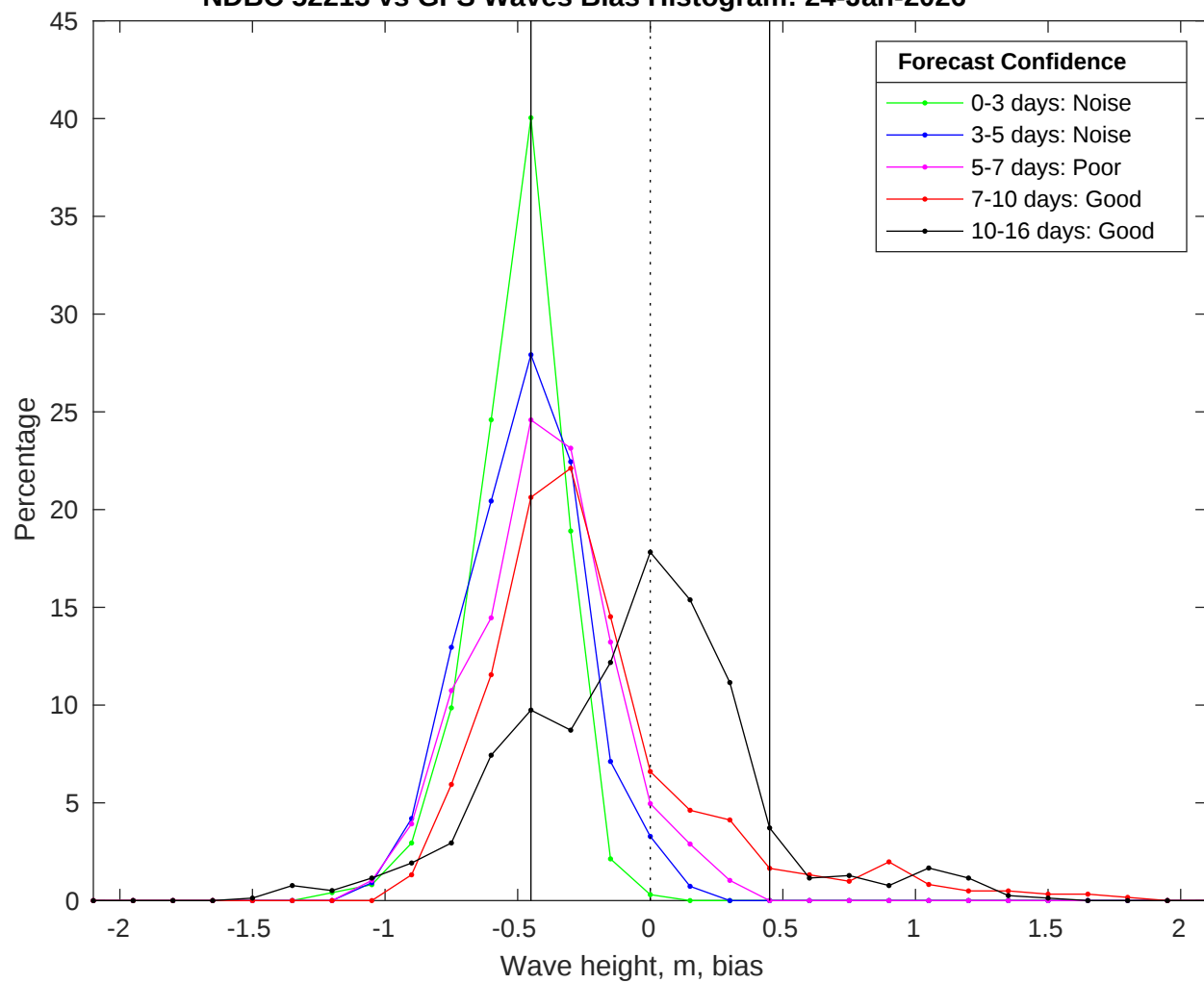
NDBC 52213 vs GFS Waves Bias Histogram: 24-Jan-2026
