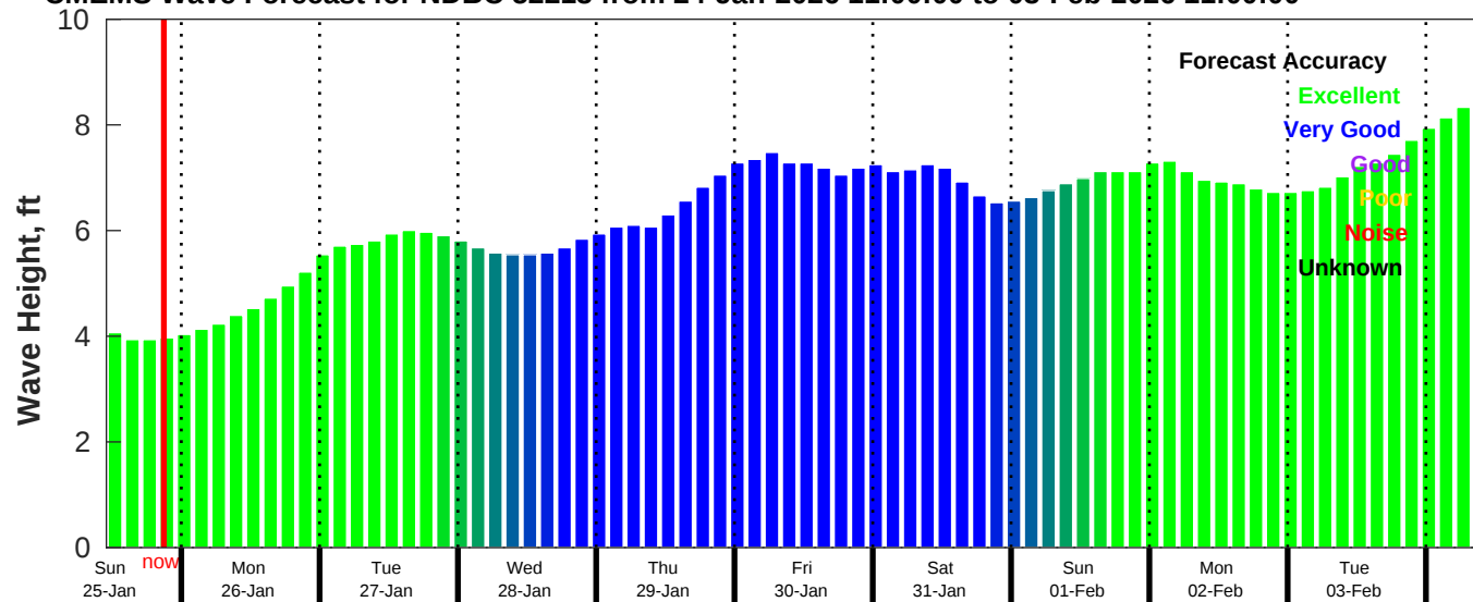
CMEMS Wave Forecast for NDBC 52213 from 24-Jan-2026 11:00:00 to 03-Feb-2026 11:00:00
