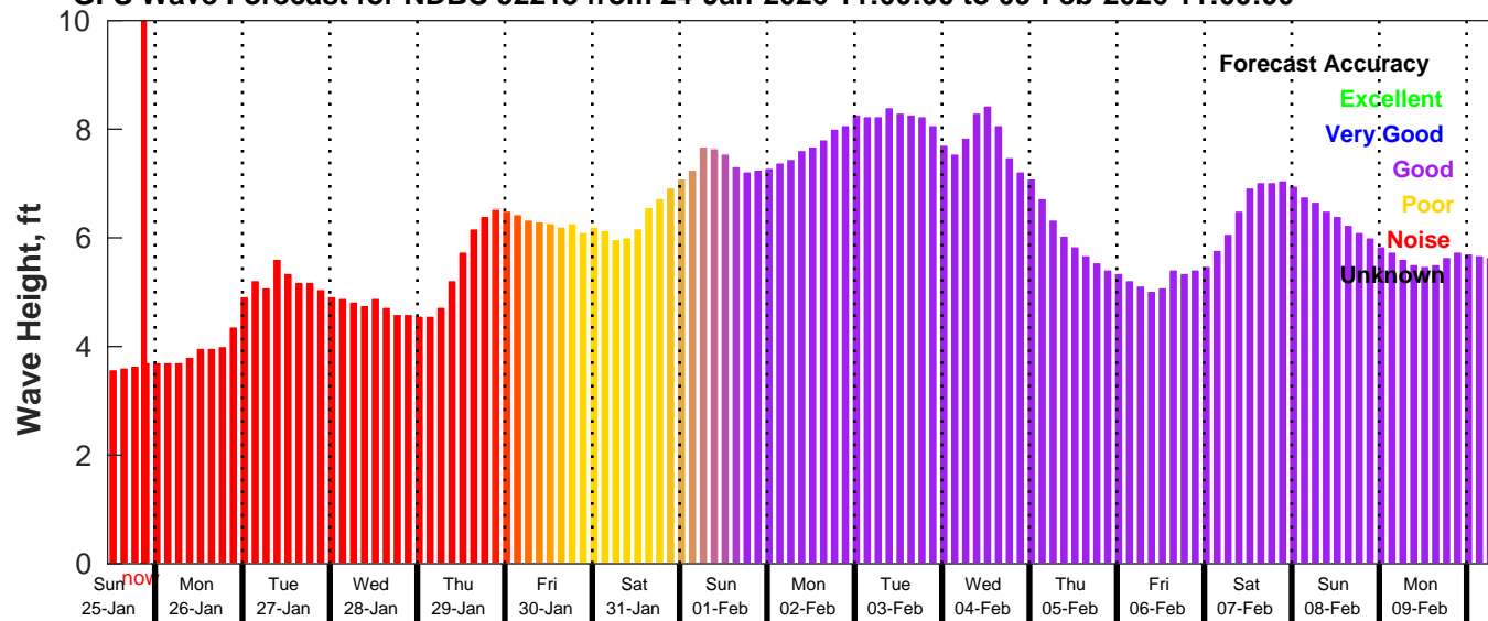
GFS Wave Forecast for NDBC 52213 from 24-Jan-2026 11:00:00 to 09-Feb-2026 11:00:00
