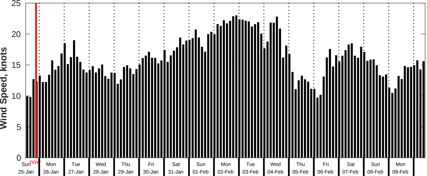
GFS Wind Speed Forecast for NDBC 52213 from 24-Jan-2026 11:00:00 to 09-Feb-2026 11:00:00
