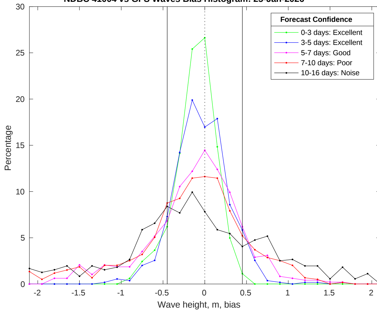
NDBC 41004 vs GFS Waves Bias Histogram: 25-Jan-2026
