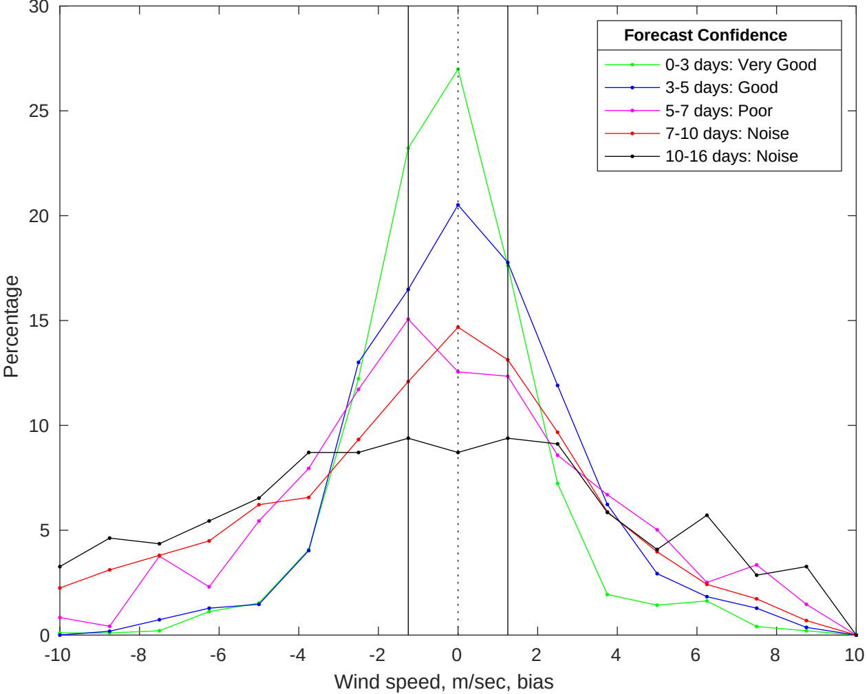
NDBC 41004 vs GFS Winds Bias Histogram: 25-Jan-2026
