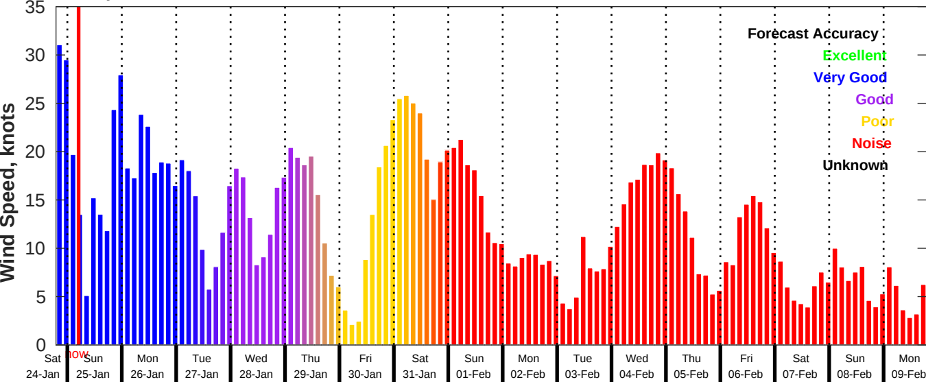
GFS Wind Speed Forecast for NDBC 41004 from 24-Jan-2026 19:00:00 to 09-Feb-2026 19:00:00
