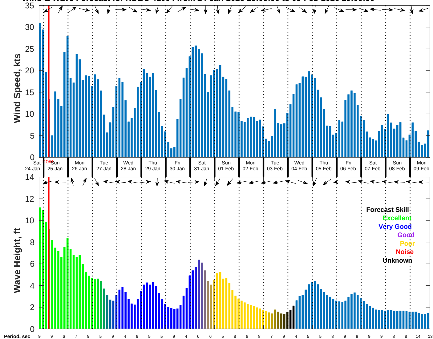
Wind & Wave Forecast for NDBC 41004 from 24-Jan-2026 19:00:00 to 09-Feb-2026 19:00:00
