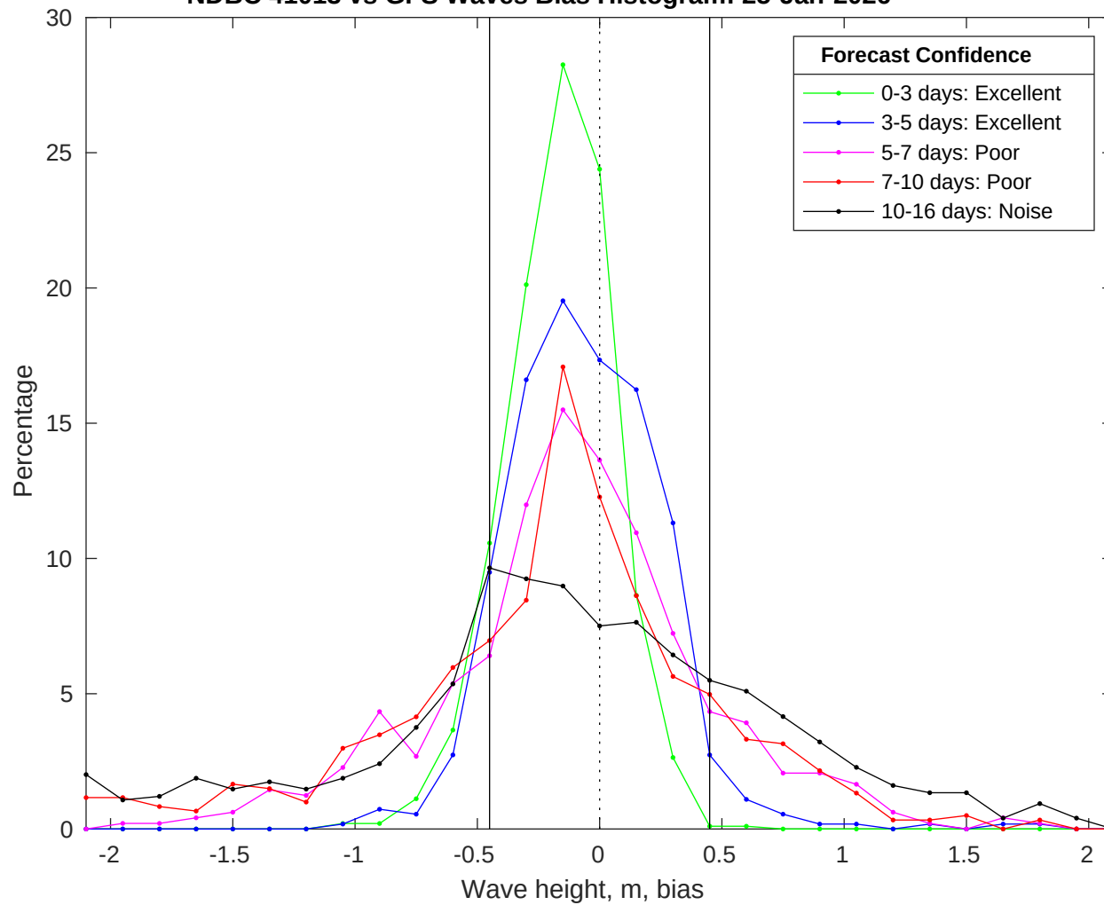
NDBC 41013 vs GFS Waves Bias Histogram: 25-Jan-2026
