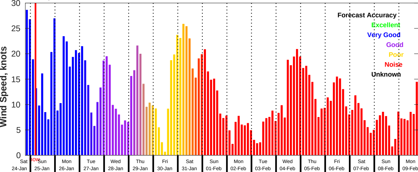
GFS Wind Speed Forecast for NDBC 41013 from 24-Jan-2026 19:00:00 to 09-Feb-2026 19:00:00
