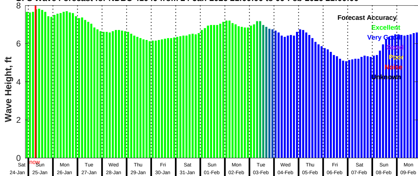
GFS Wave Forecast for NDBC 41040 from 24-Jan-2026 21:00:00 to 09-Feb-2026 21:00:00
