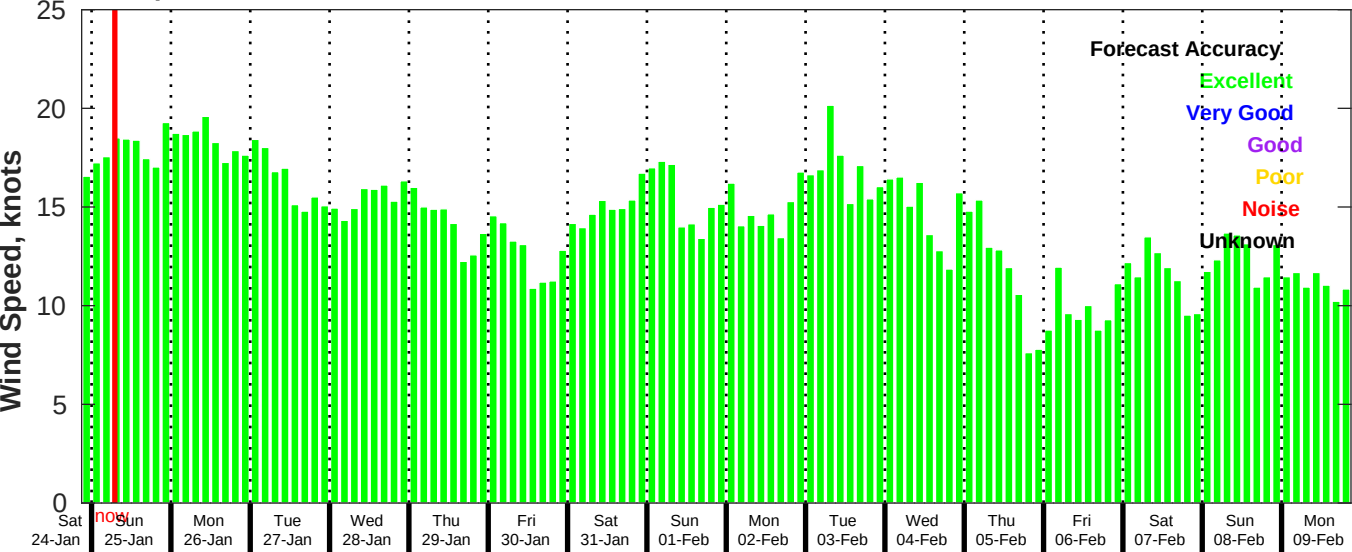
GFS Wind Speed Forecast for NDBC 41040 from 24-Jan-2026 21:00:00 to 09-Feb-2026 21:00:00
