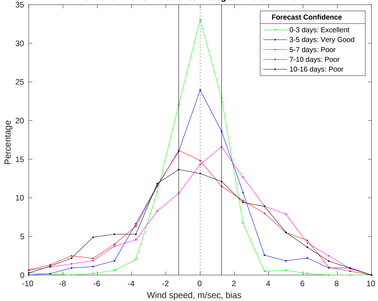
NDBC 42019 vs GFS Winds Bias Histogram: 25-Jan-2026
