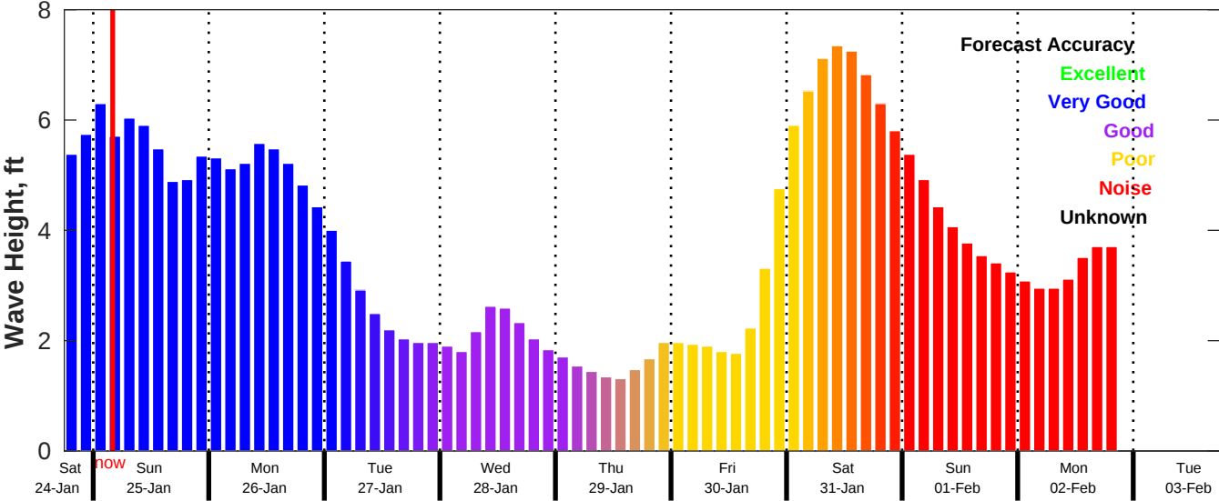
CMEMS Wave Forecast for NDBC 42019 from 24-Jan-2026 18:00:00 to 03-Feb-2026 18:00:00
