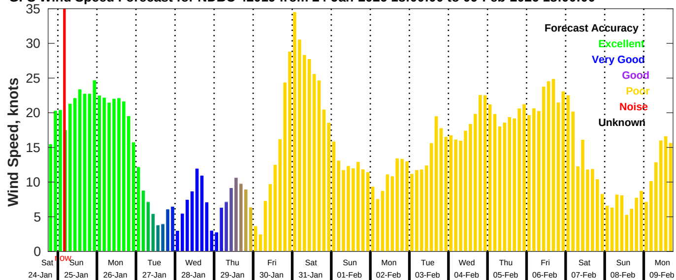
GFS Wind Speed Forecast for NDBC 42019 from 24-Jan-2026 18:00:00 to 09-Feb-2026 18:00:00
