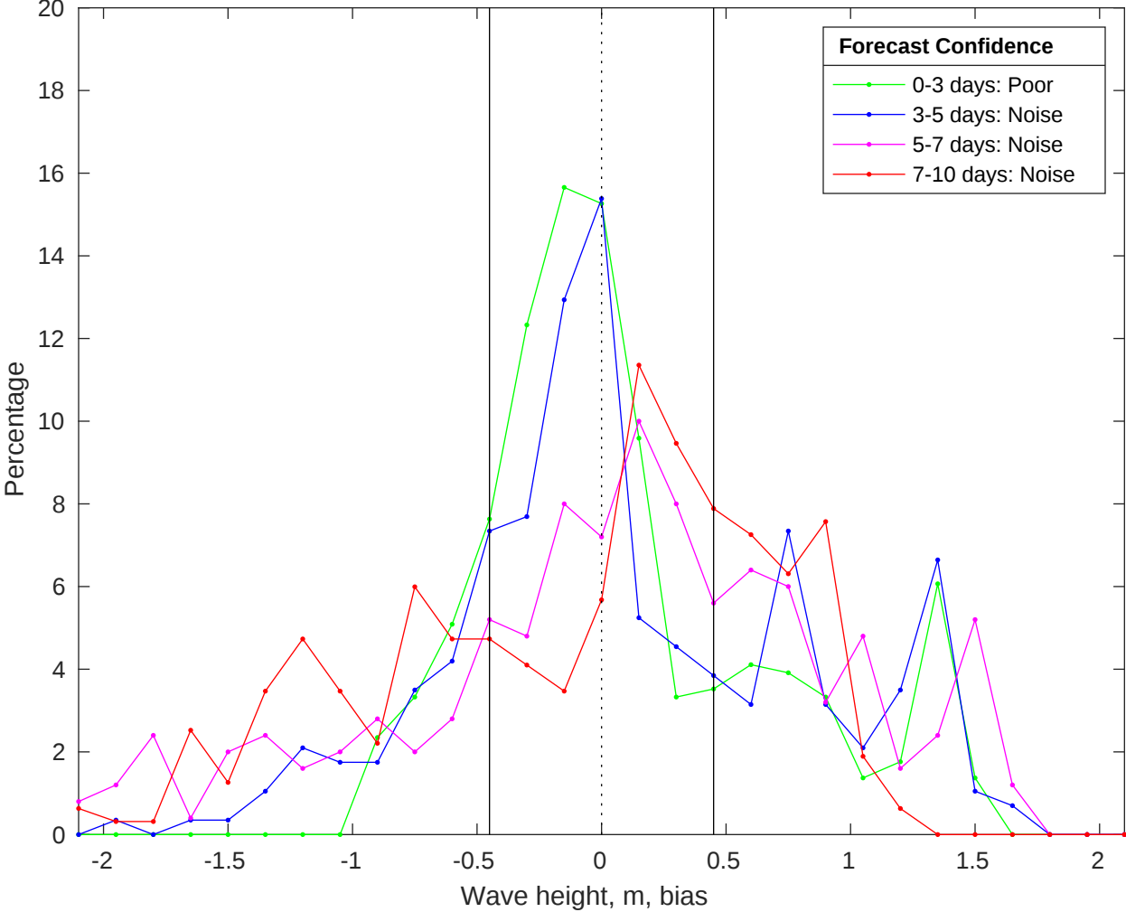
NDBC 42020 vs CMEMS Waves Bias Histogram: 25-Jan-2026
