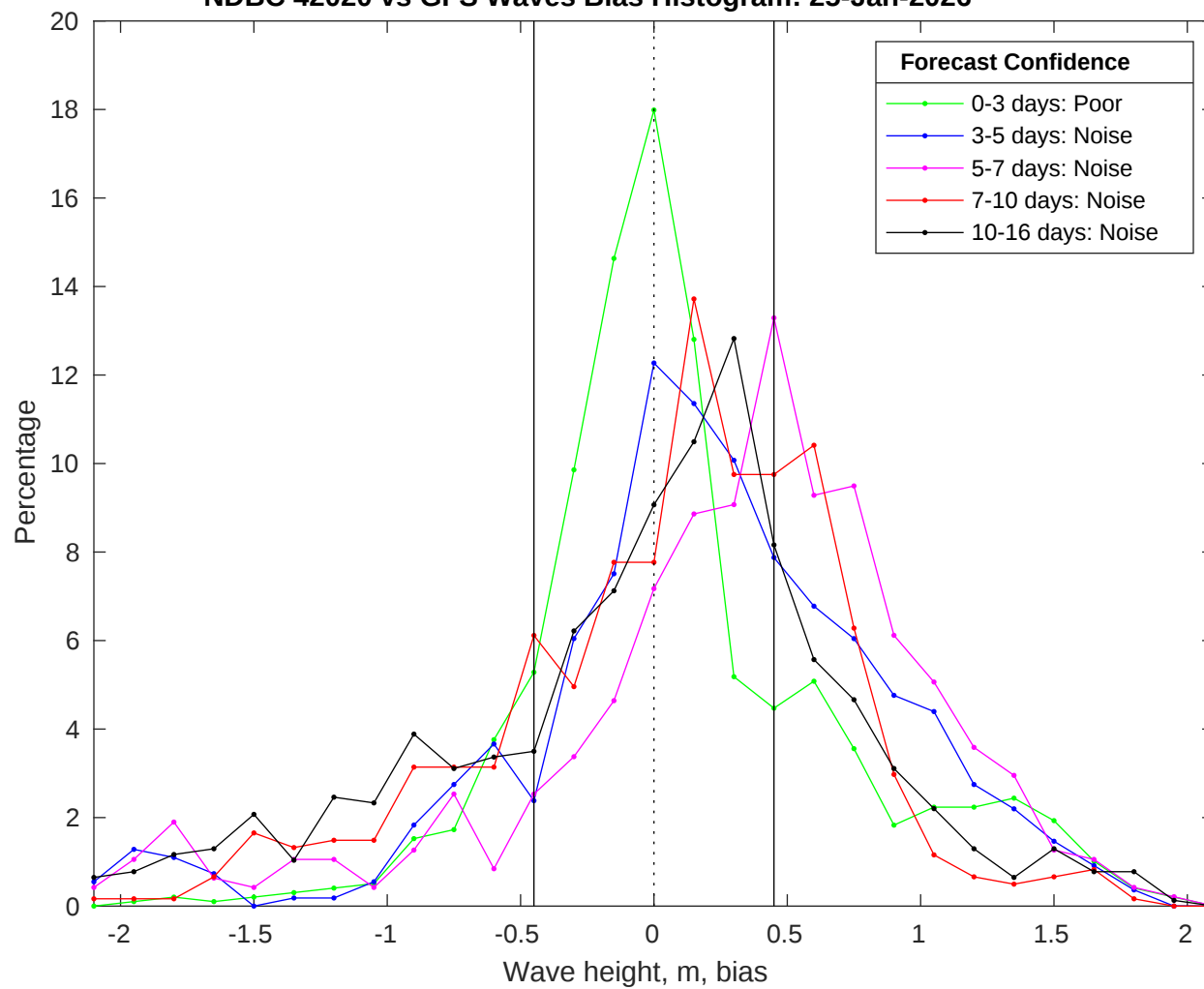
NDBC 42020 vs GFS Waves Bias Histogram: 25-Jan-2026
