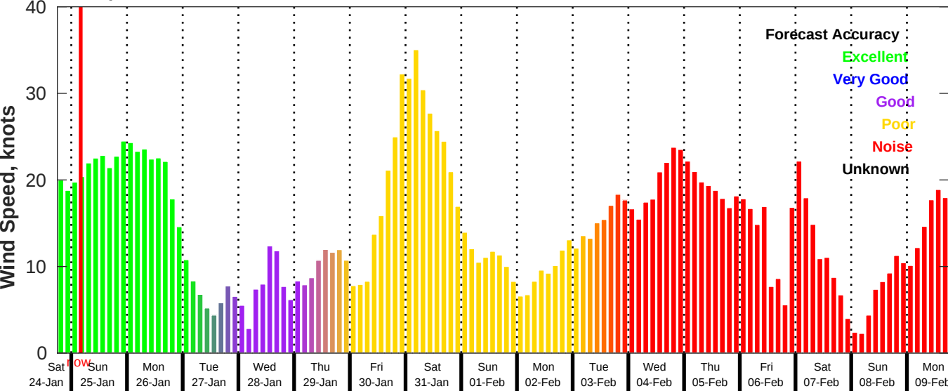
GFS Wind Speed Forecast for NDBC 42020 from 24-Jan-2026 18:00:00 to 09-Feb-2026 18:00:00
