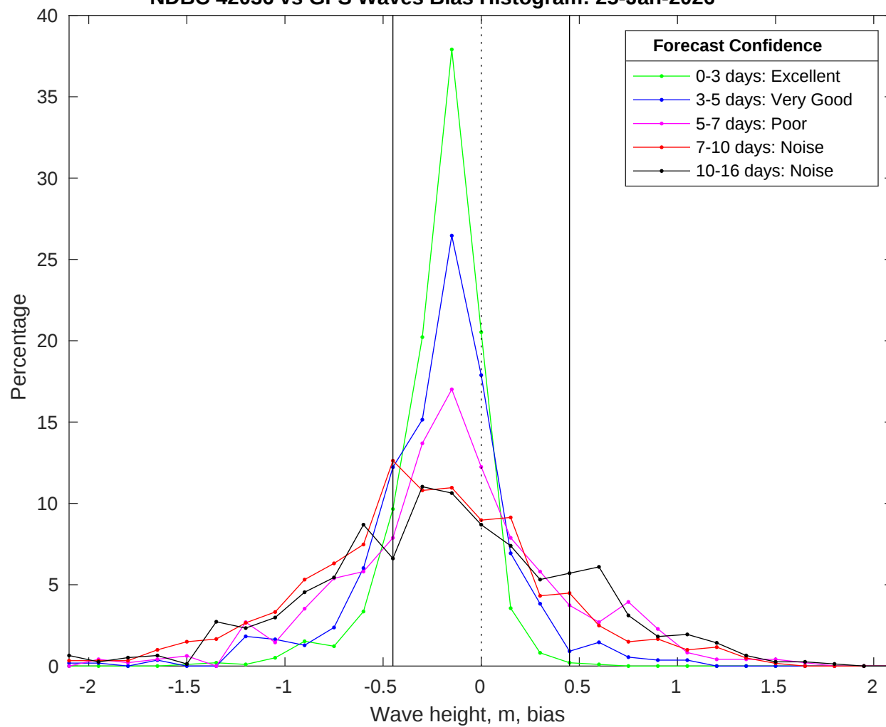
NDBC 42036 vs GFS Waves Bias Histogram: 25-Jan-2026
