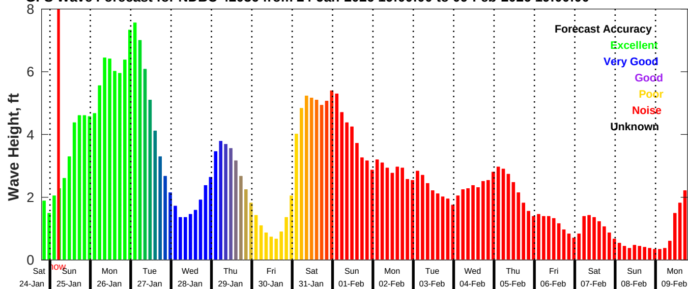
GFS Wave Forecast for NDBC 42036 from 24-Jan-2026 19:00:00 to 09-Feb-2026 19:00:00
