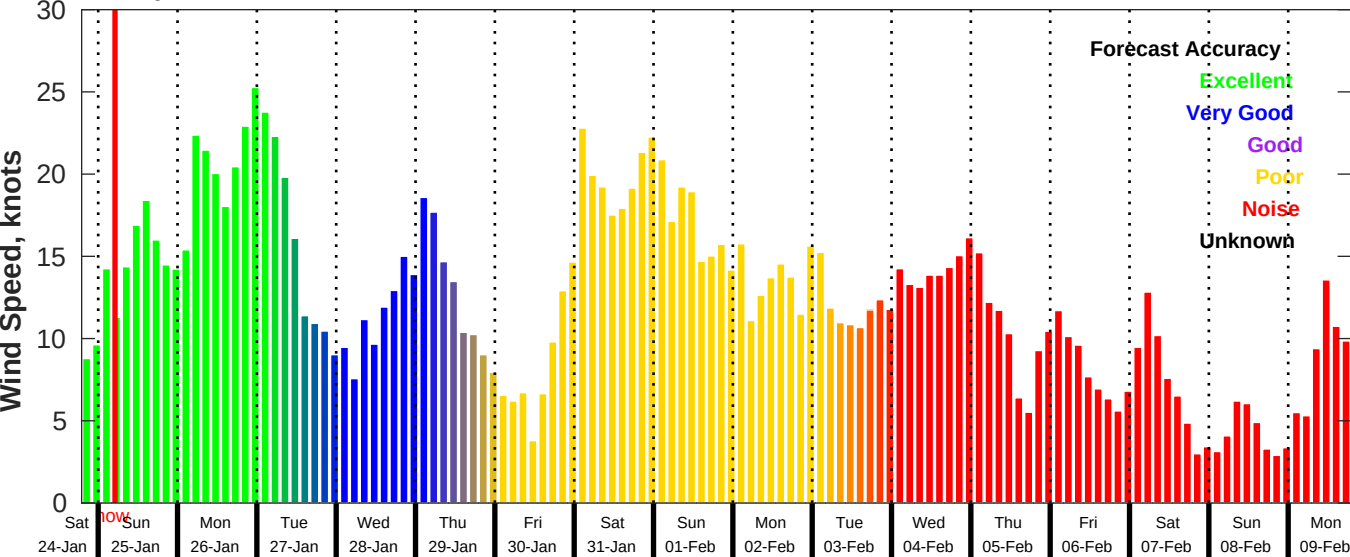
GFS Wind Speed Forecast for NDBC 42036 from 24-Jan-2026 19:00:00 to 09-Feb-2026 19:00:00
