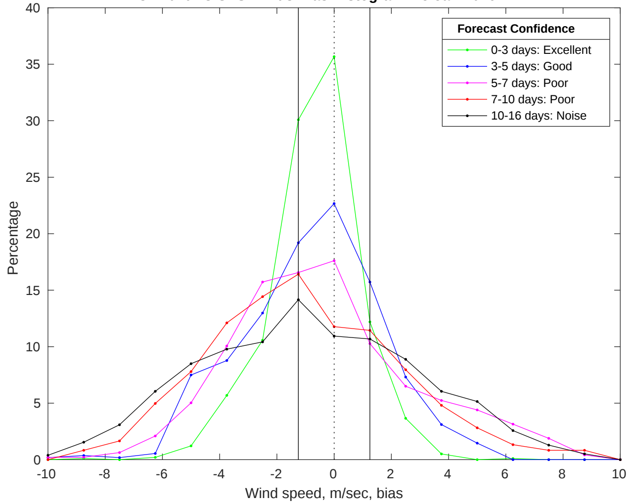
NDBC 42040 vs GFS Winds Bias Histogram: 25-Jan-2026
