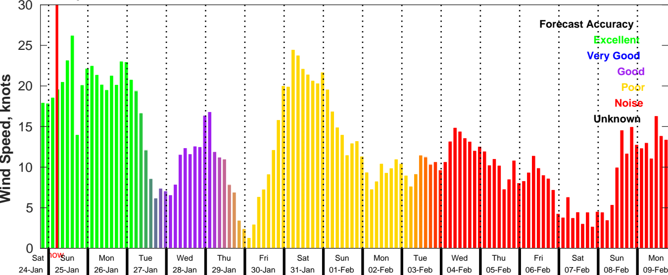
GFS Wind Speed Forecast for NDBC 42040 from 24-Jan-2026 19:00:00 to 09-Feb-2026 19:00:00
