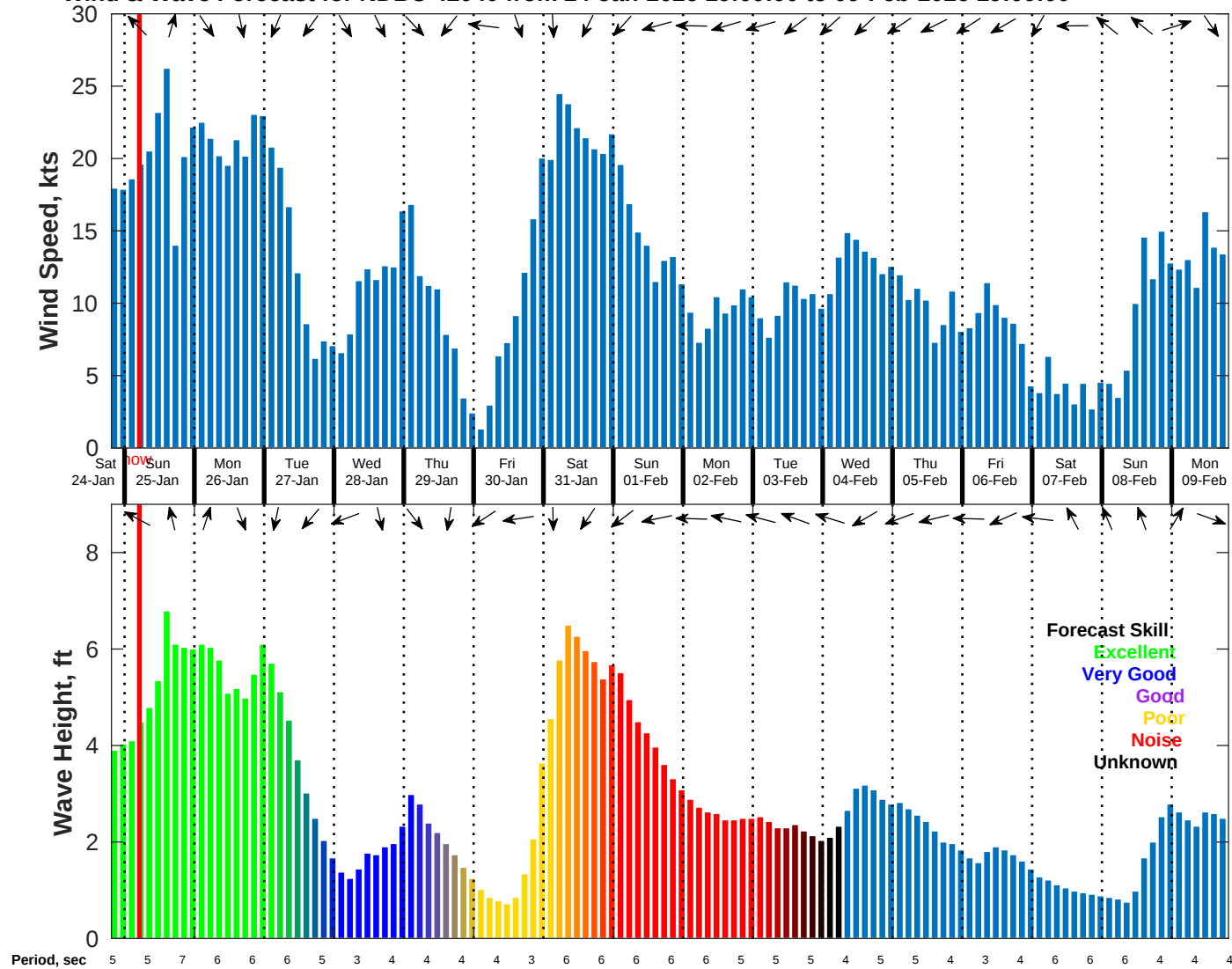
Wind & Wave Forecast for NDBC 42040 from 24-Jan-2026 19:00:00 to 09-Feb-2026 19:00:00
