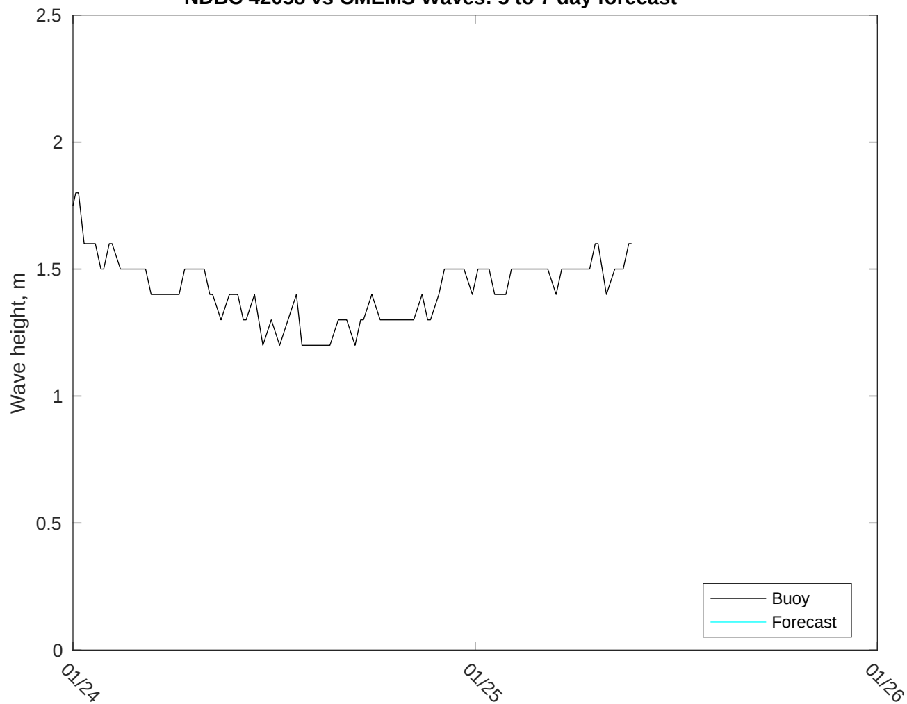
NDBC 42058 vs CMEMS Waves: 5 to 7 day forecast
