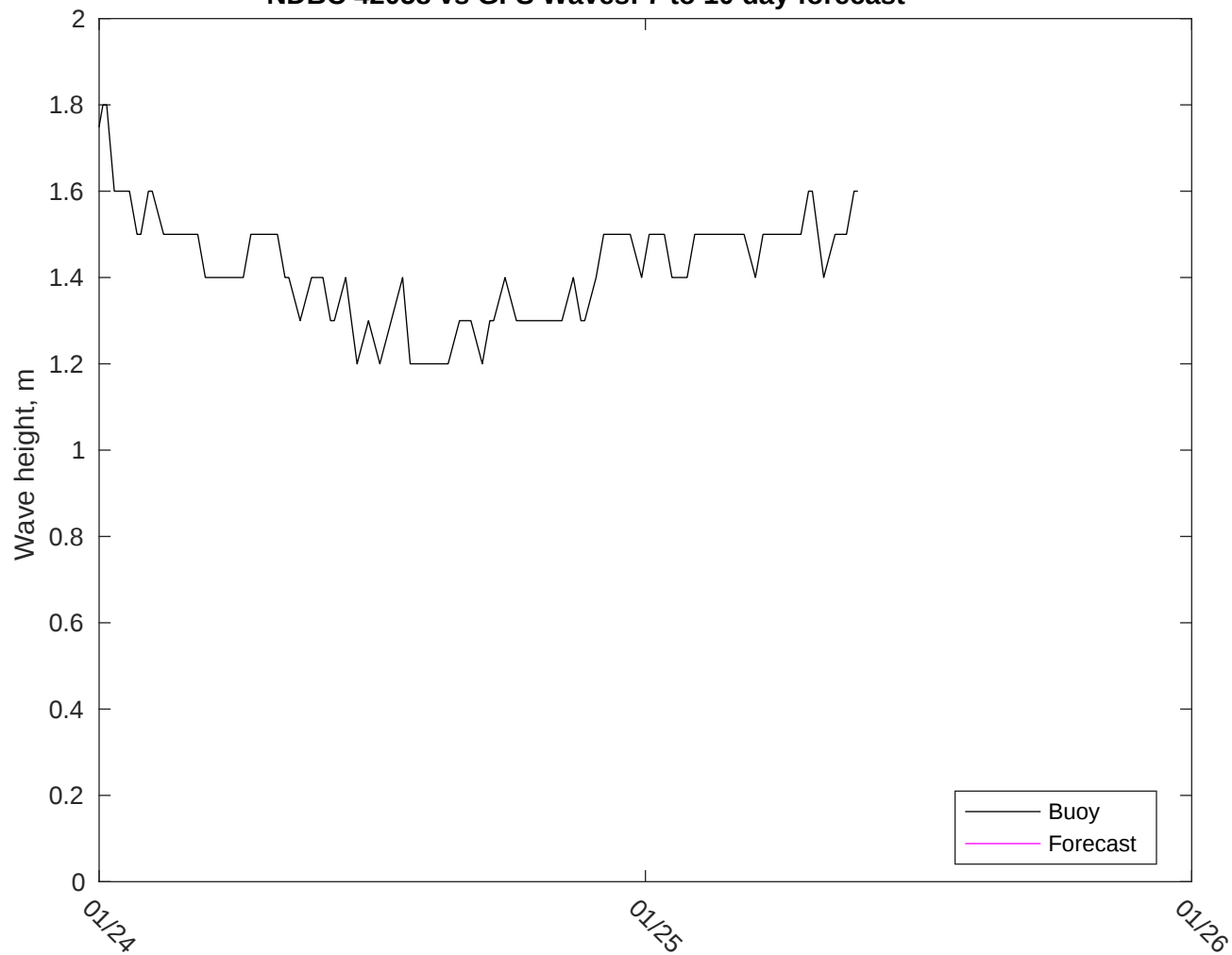
NDBC 42058 vs GFS Waves: 7 to 10 day forecast
