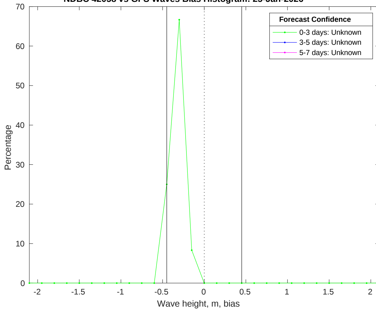
NDBC 42058 vs GFS Waves Bias Histogram: 25-Jan-2026
