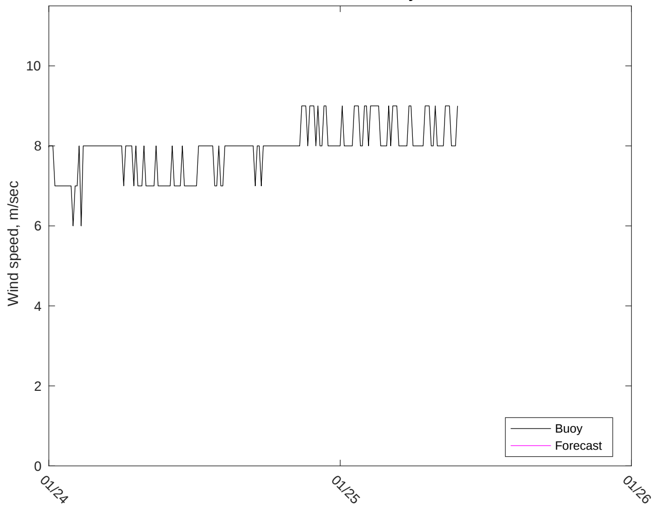
NDBC 42058 vs GFS Winds: 7 to 10 day forecast
