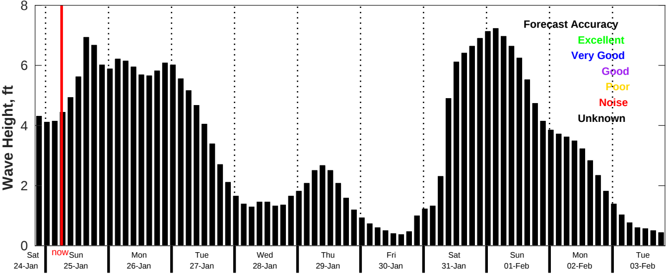
CMEMS Wave Forecast for NDBC 42058 from 24-Jan-2026 20:00:00 to 03-Feb-2026 20:00:00
