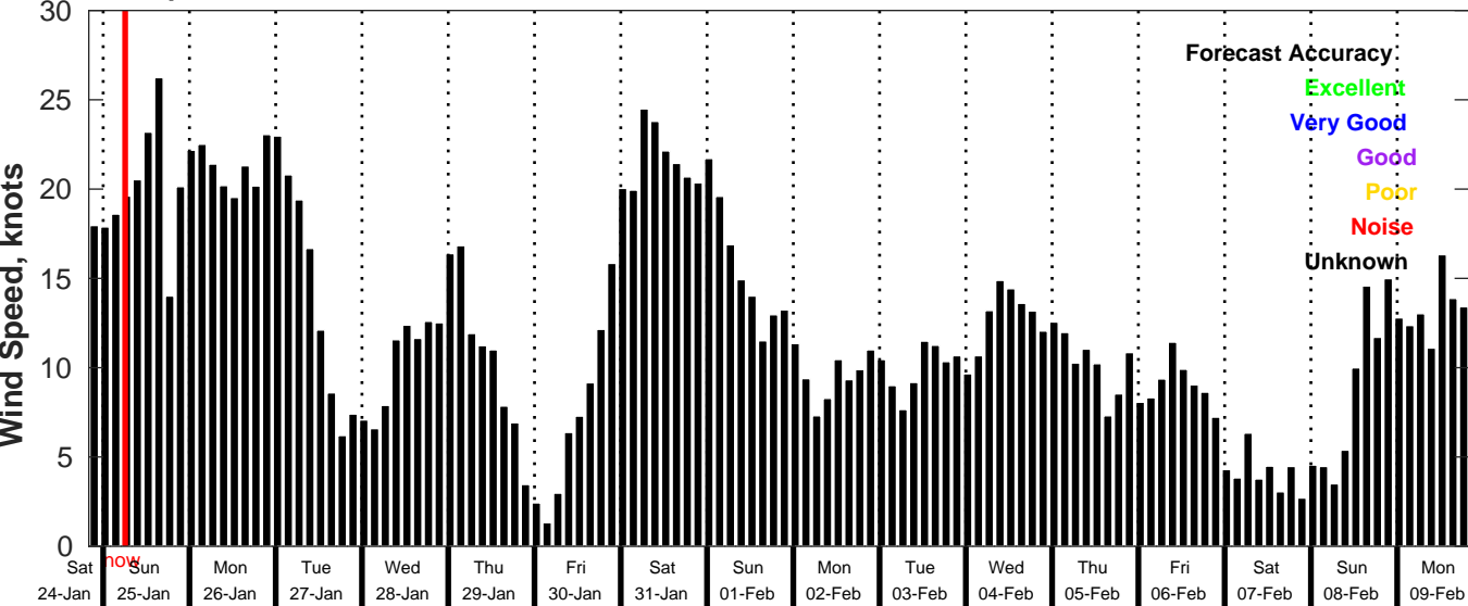
GFS Wind Speed Forecast for NDBC 42058 from 24-Jan-2026 20:00:00 to 09-Feb-2026 20:00:00
