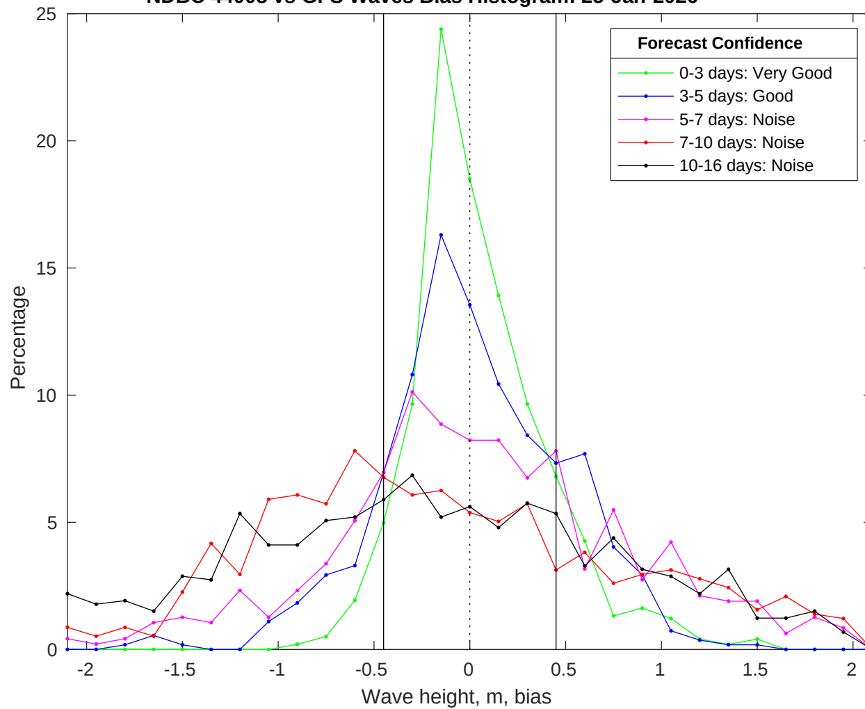
NDBC 44008 vs GFS Waves Bias Histogram: 25-Jan-2026
