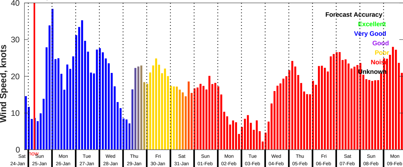
GFS Wind Speed Forecast for NDBC 44008 from 24-Jan-2026 20:00:00 to 09-Feb-2026 20:00:00
