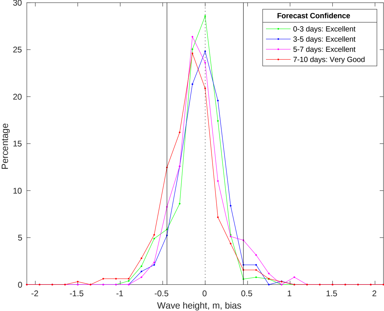
NDBC 46011 vs CMEMS Waves Bias Histogram: 25-Jan-2026
