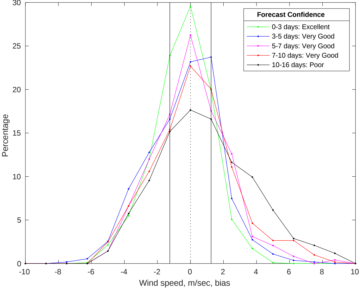
NDBC 46011 vs GFS Winds Bias Histogram: 25-Jan-2026
