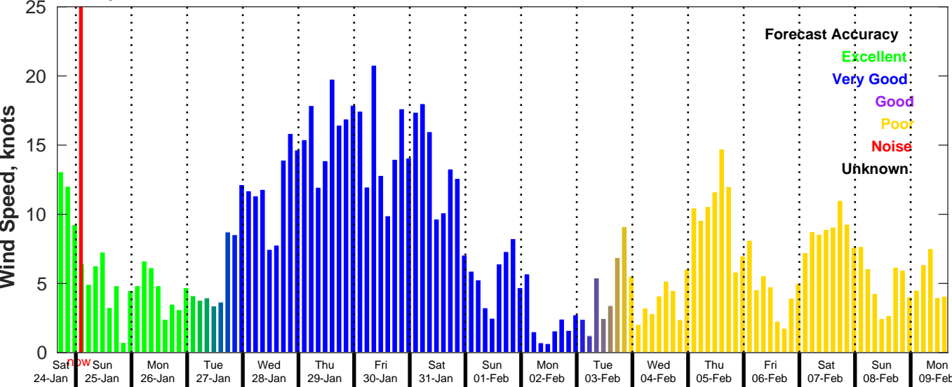
GFS Wind Speed Forecast for NDBC 46011 from 24-Jan-2026 16:00:00 to 09-Feb-2026 16:00:00
