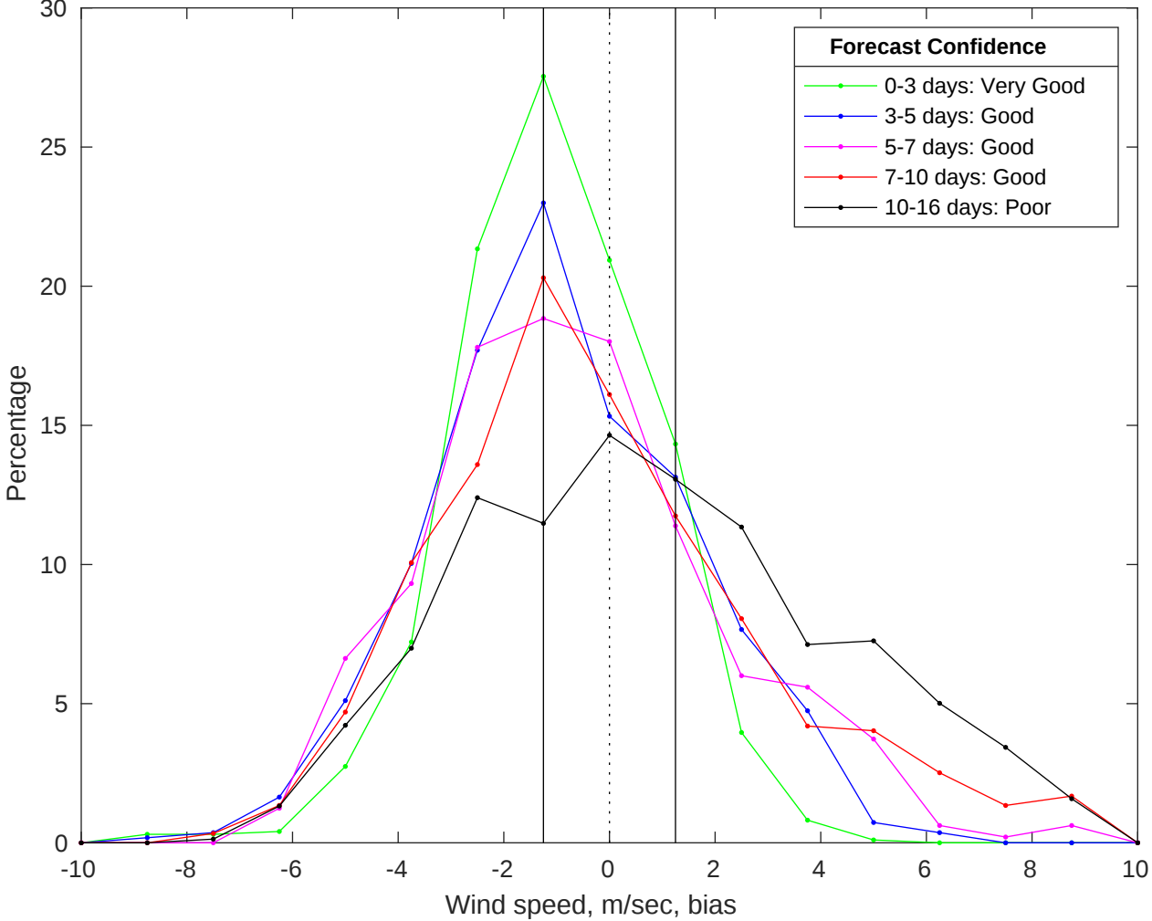
NDBC 46028 vs GFS Winds Bias Histogram: 25-Jan-2026
