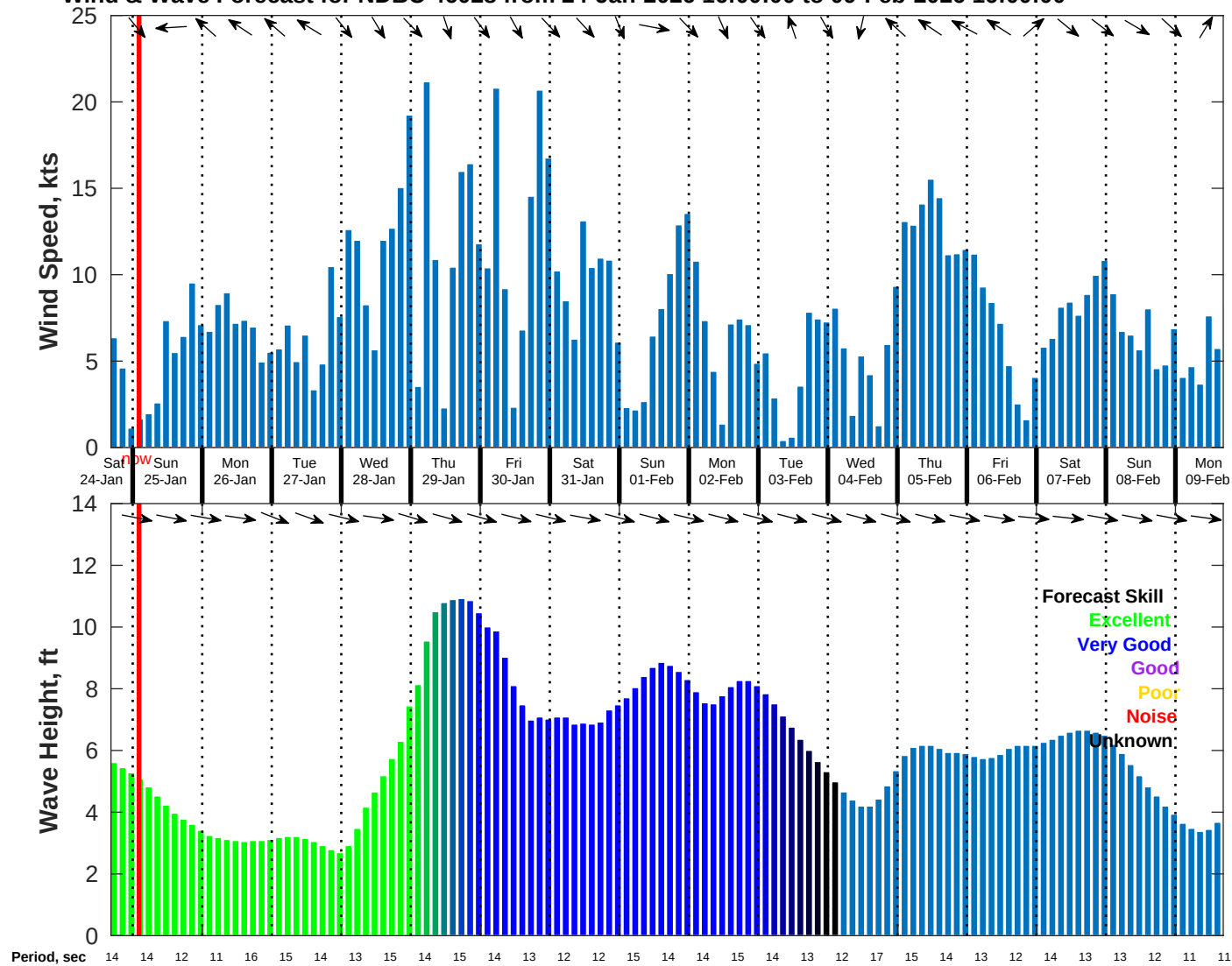
Wind & Wave Forecast for NDBC 46028 from 24-Jan-2026 16:00:00 to 09-Feb-2026 16:00:00
