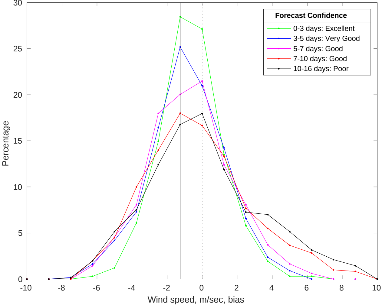
NDBC 46054 vs GFS Winds Bias Histogram: 25-Jan-2026
