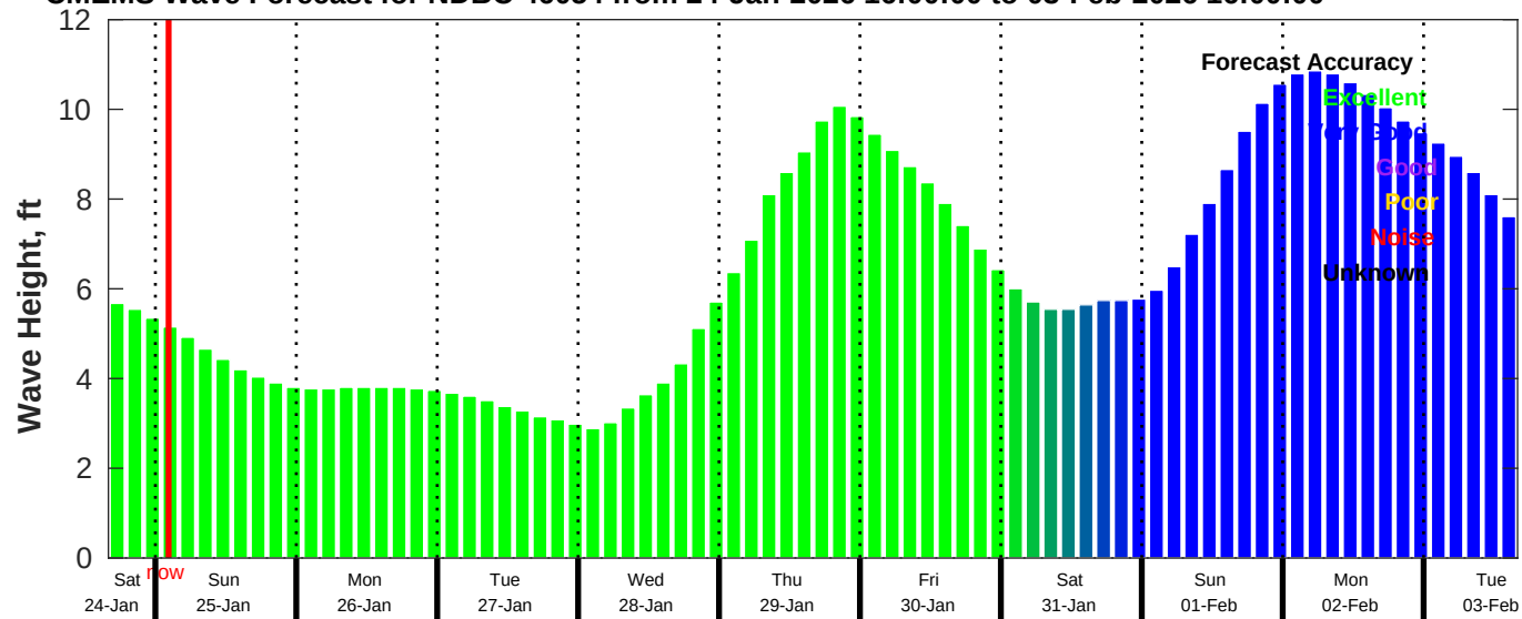
CMEMS Wave Forecast for NDBC 46054 from 24-Jan-2026 16:00:00 to 03-Feb-2026 16:00:00
