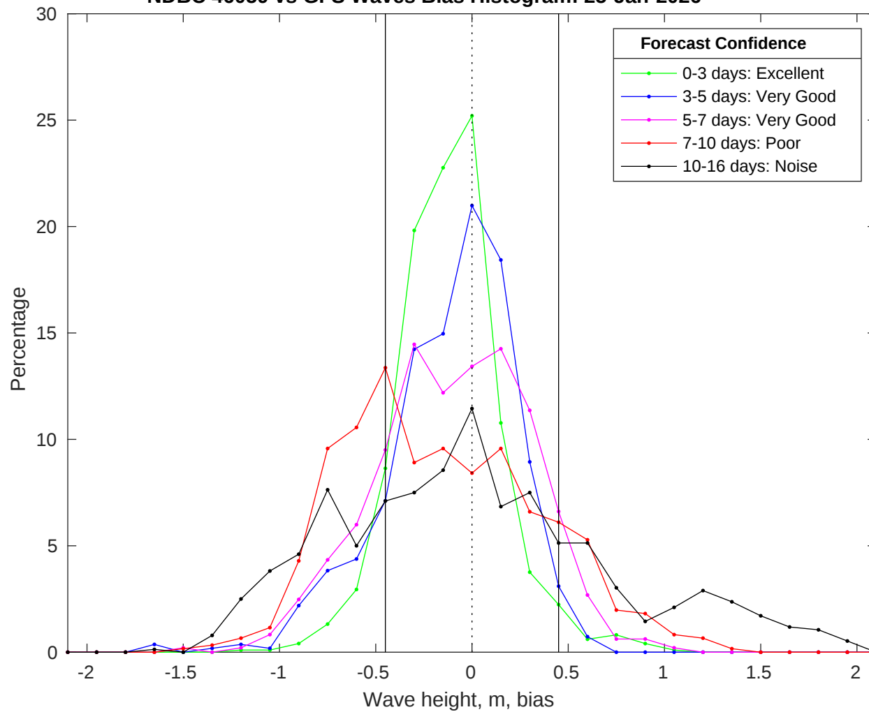
NDBC 46059 vs GFS Waves Bias Histogram: 25-Jan-2026
