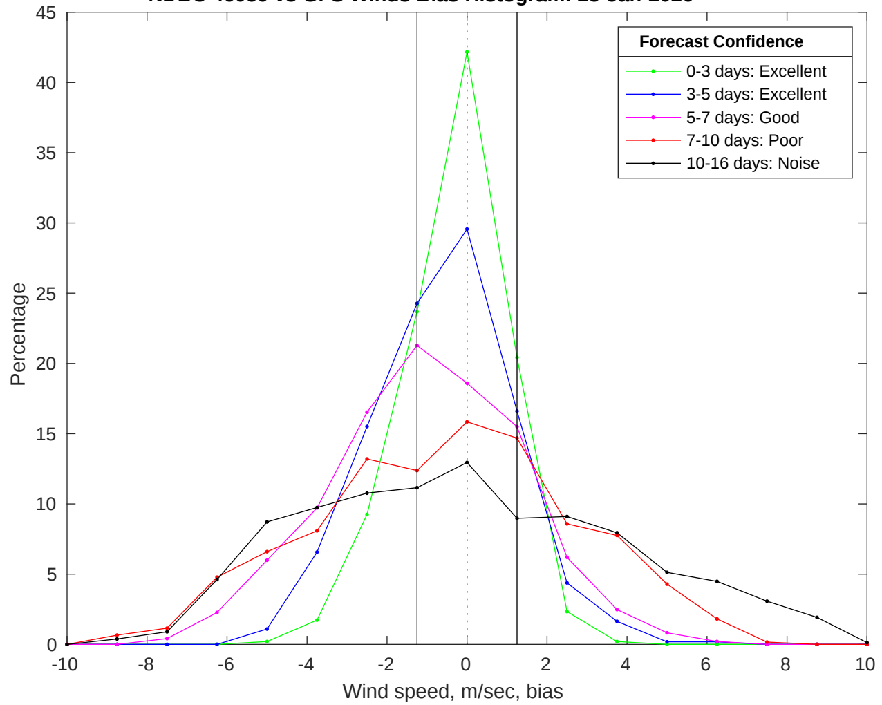
NDBC 46059 vs GFS Winds Bias Histogram: 25-Jan-2026
