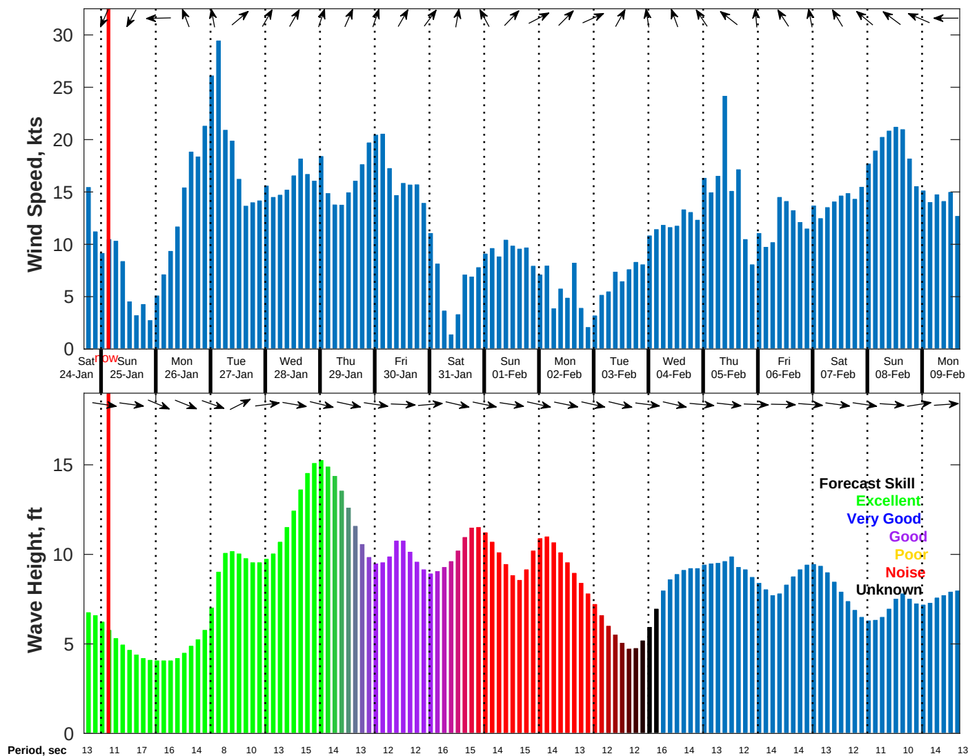
Wind & Wave Forecast for NDBC 46059 from 24-Jan-2026 17:00:00 to 09-Feb-2026 17:00:00
